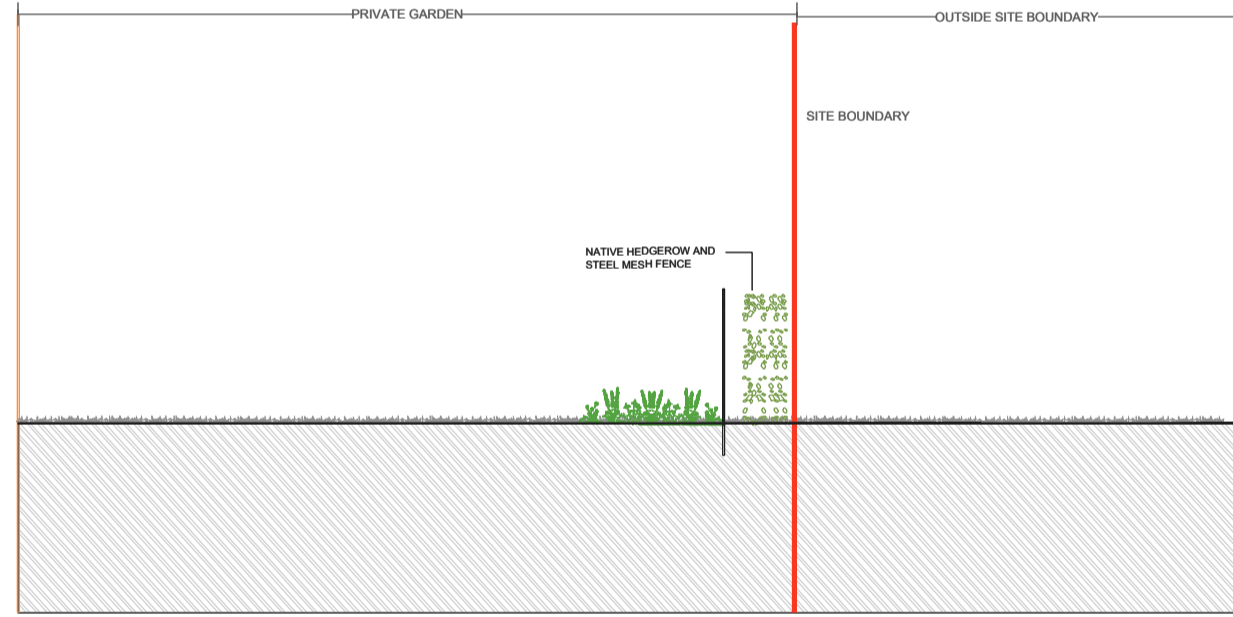
B5 PROPOSED NATIVE HEDGEROW AND STEEL MESH FENCE SCALE: 1:100 @ A1
