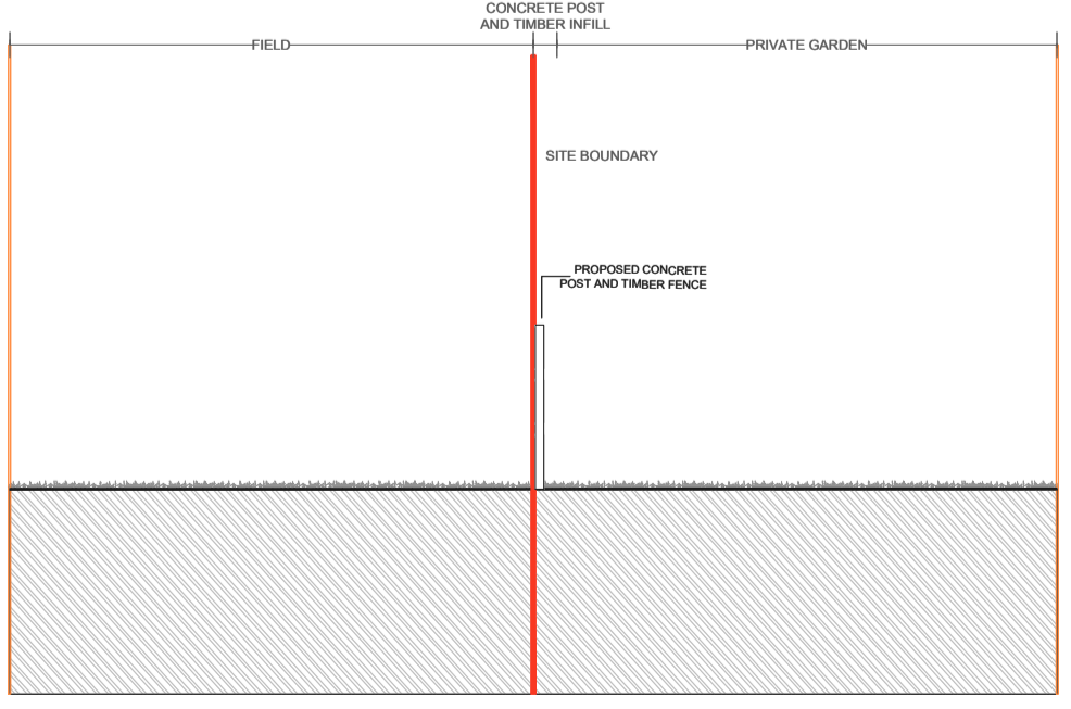
B12 CONCRETE POST AND TIMBER FENCE SCALE: 1:100 @ A1
