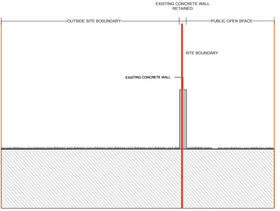
B19 EXISTING CONCRETE WALL RETAINED SCALE: 1:100 @ A1
