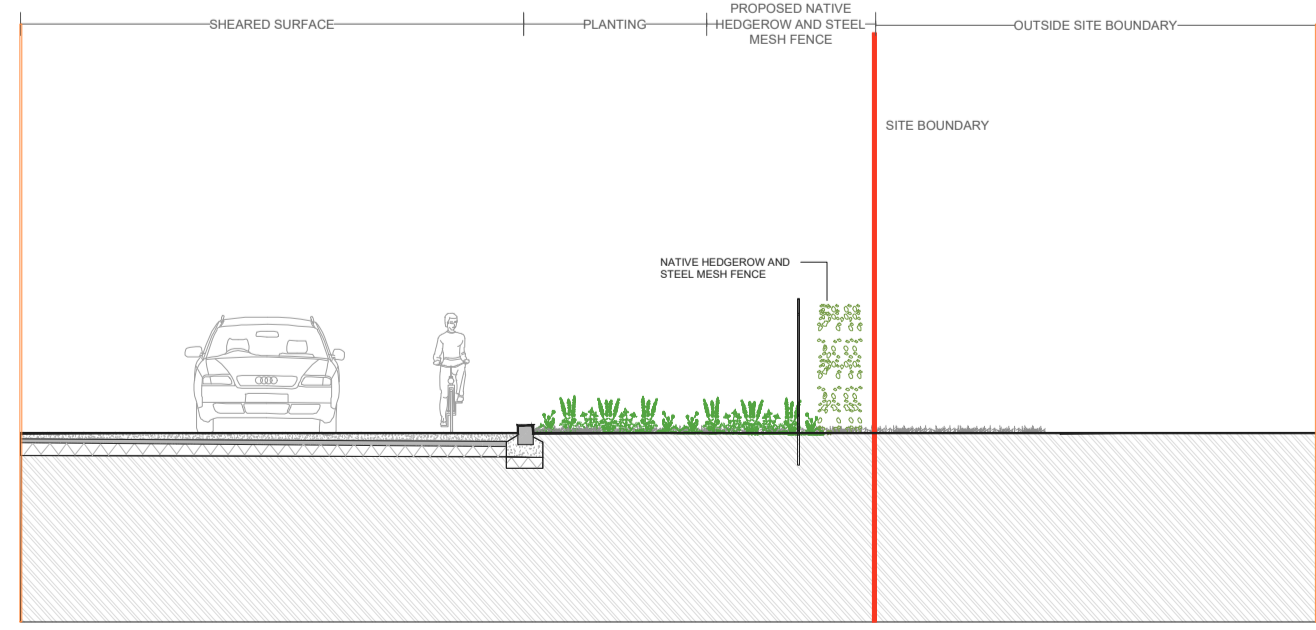
B10 PROPOSED NATIVE HEDGEROW AND STEEL MESH FENCE SCALE: 1:100 @ A1
