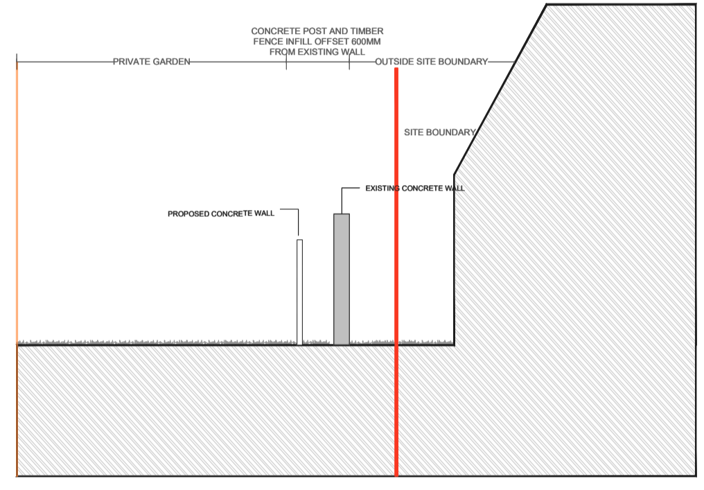
B18 CONCRETE POST AND TIMBER FENCE INFILL OFFSET 600MM FROM EXISTING WALL SCALE: 1:100 @ A1
