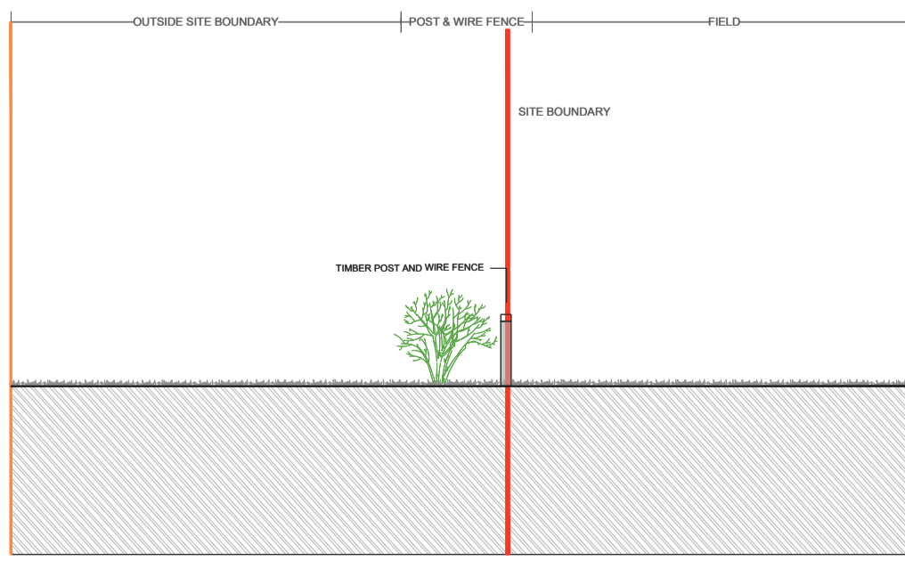
B12 EXISTING POST AND WIRE FENCE SCALE: 1:100 @ A1
