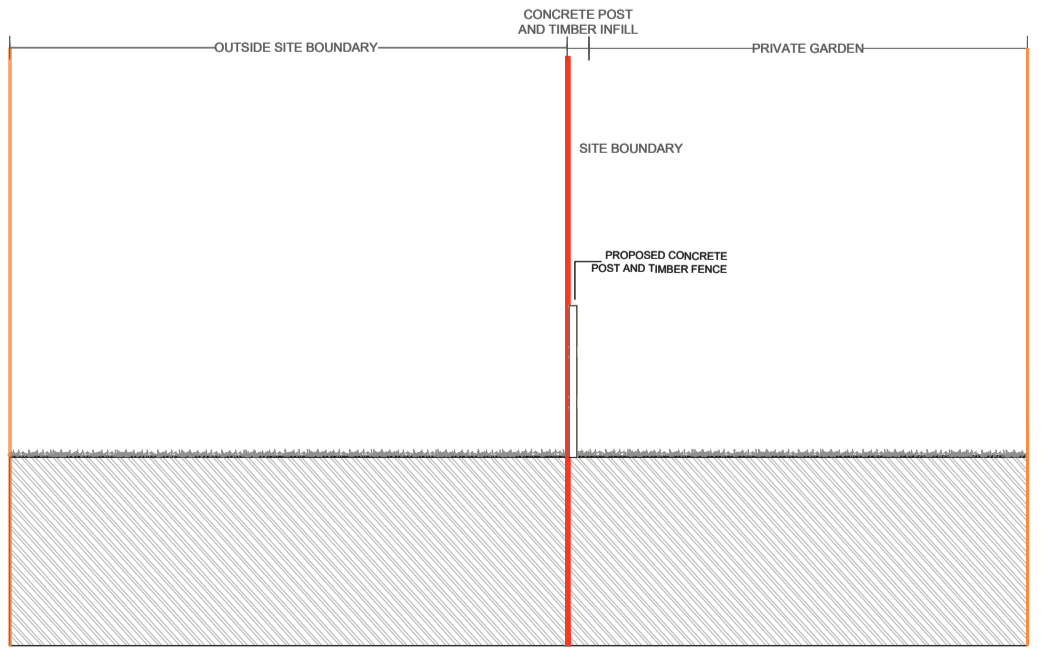
B13 CONCRETE POST AND TIMBER INFILL SCALE: 1:100 @ A1
